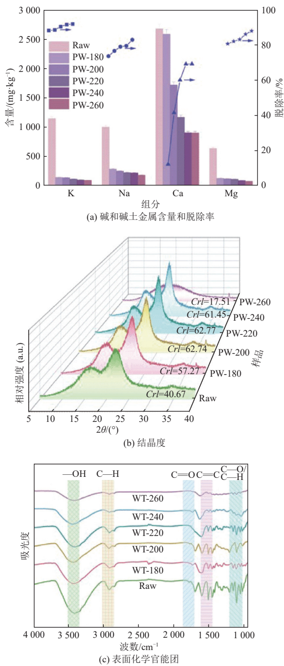
图3 温度对杨木湿法烘焙固体产物化学结构的变化 [46] Fig. 3 Evolution of chemical structure of poplar wood after wet torrefaction at different temperatures [46]
